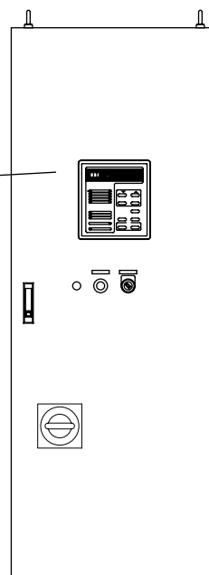
Fig. 15 - Control panel
