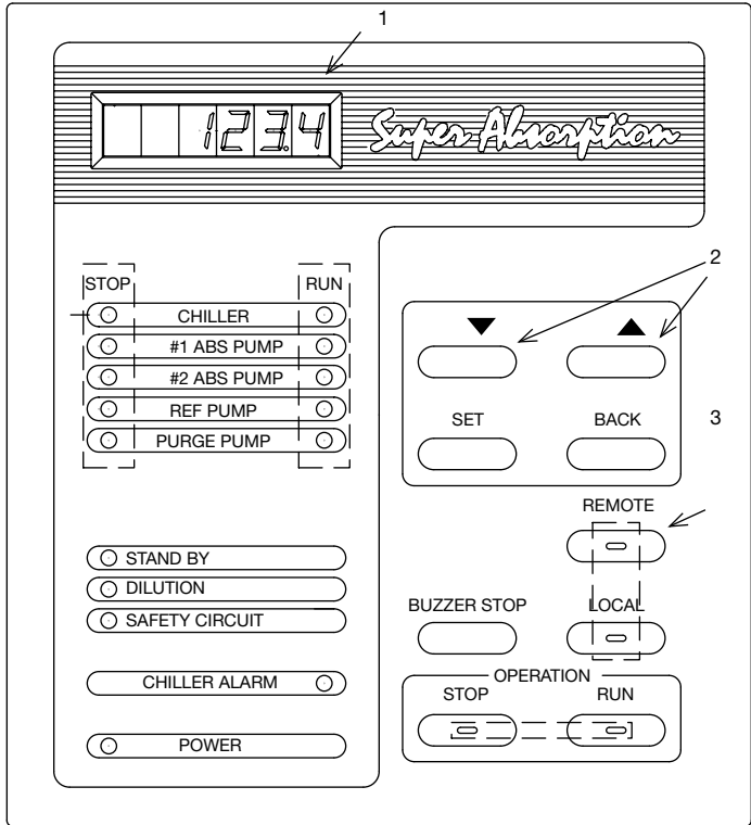
Fig. 22 - Control board
