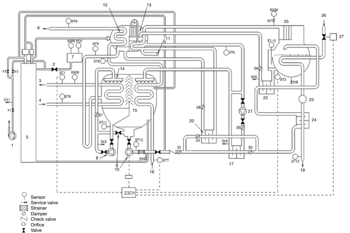
Fig. 14 - Flow diagram
