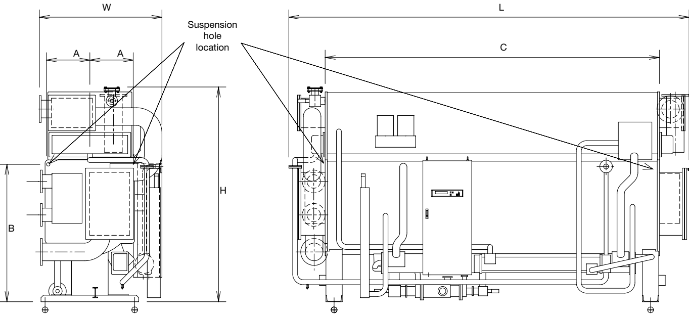
Fig. 12 - One-piece shipping
